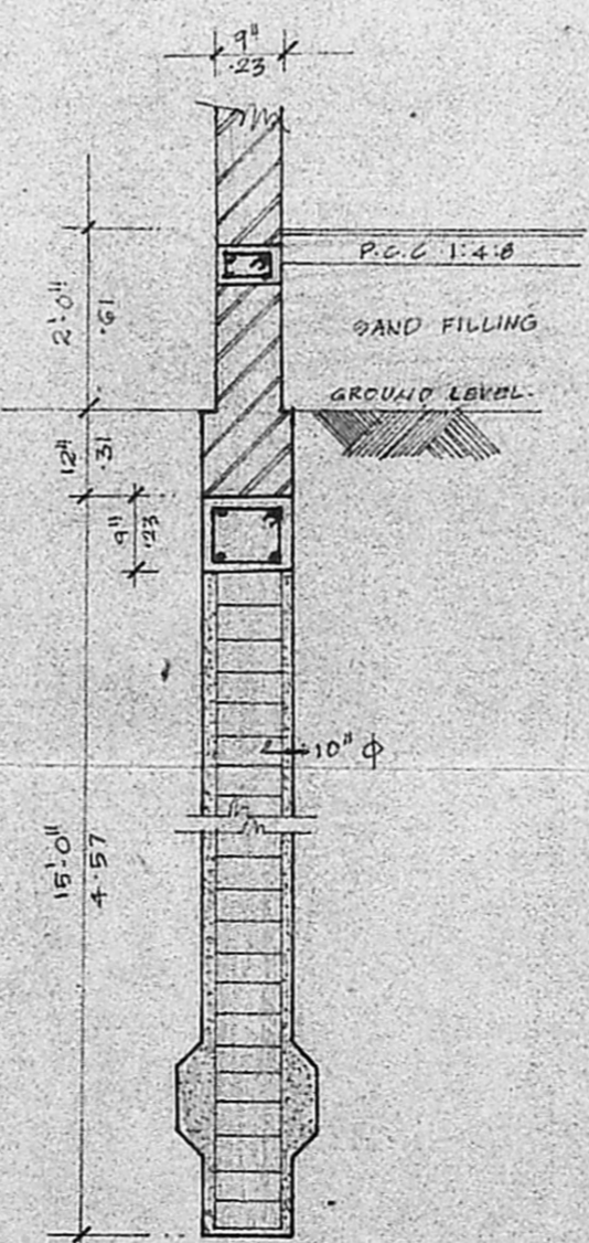
PILE FOUNDATION
